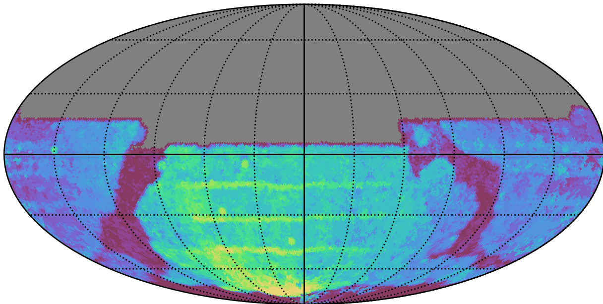
weather_cloudso10v3.4_10yrs All sky y band: Median Season Length
