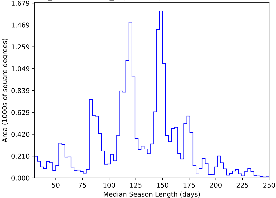
weather_cloudso10v3.4_10yrs All sky y band: Median Season Length
