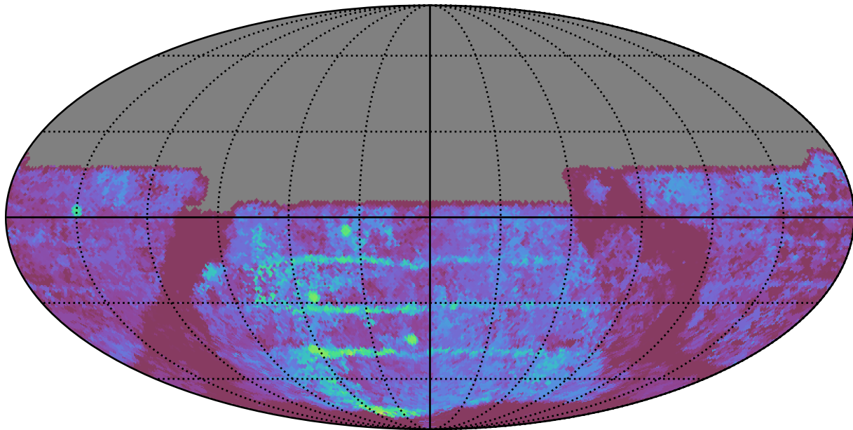
weather_cloudso10v3.4_10yrs All sky u band: Median Season Length
