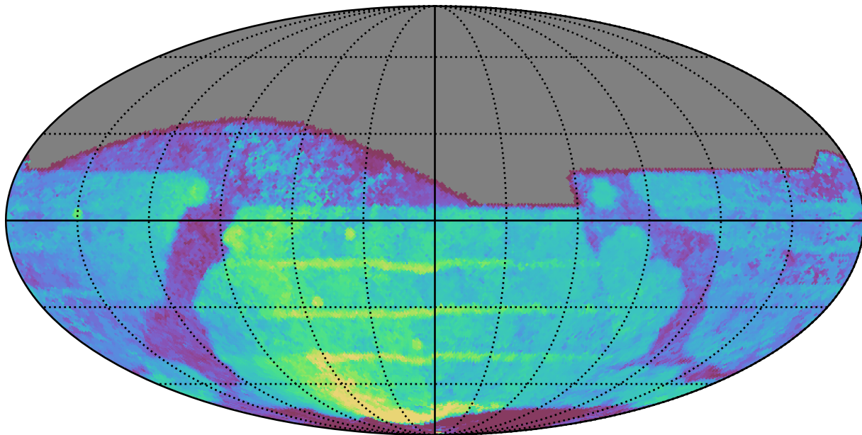
weather_cloudso10v3.4_10yrs All sky r band: Median Season Length
