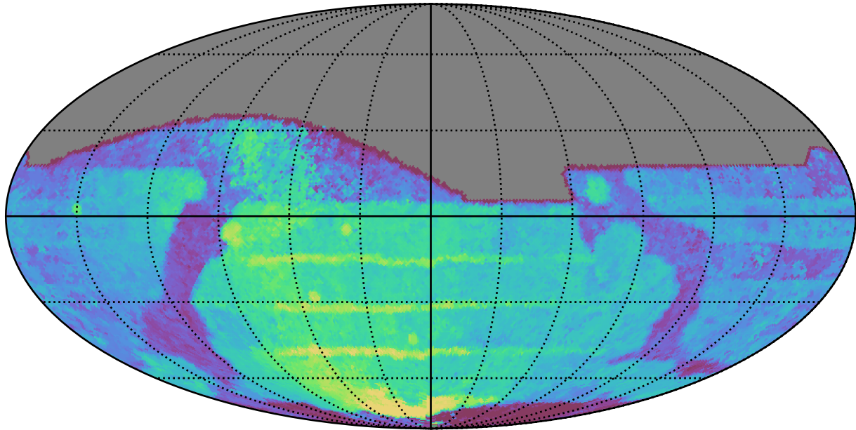
weather_cloudso10v3.4_10yrs All sky i band: Median Season Length
