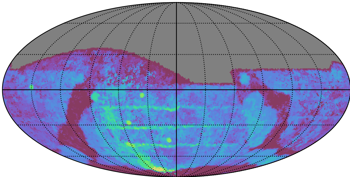
weather_cloudso10v3.4_10yrs All sky g band: Median Season Length
