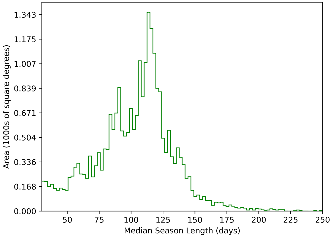
weather_cloudso10v3.4_10yrs All sky g band: Median Season Length
