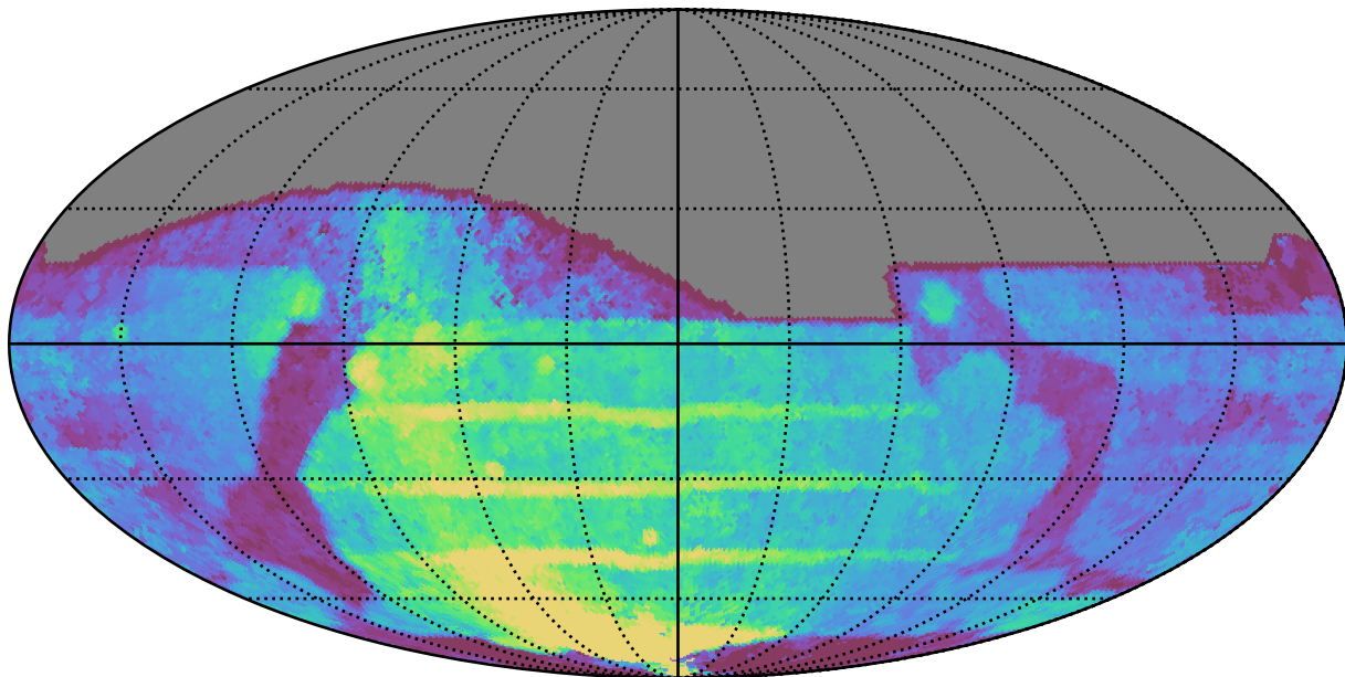
weather_cloudso10v3.4_10yrs All sky all bands: Median Season Length
