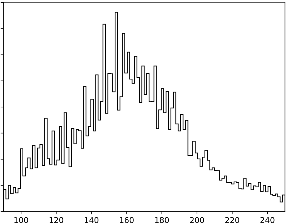
weather_cloudso10v3.4_10yrs All sky all bands: Median Season Length
