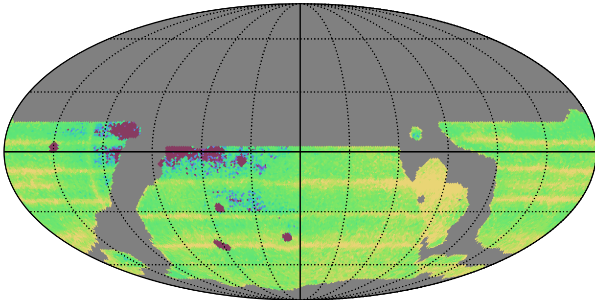
weather_cloudso10v3.4_10yrs WFD: Median Intra-Night Gap
