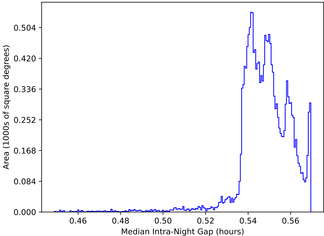
weather_cloudso10v3.4_10yrs WFD: Median Intra-Night Gap
