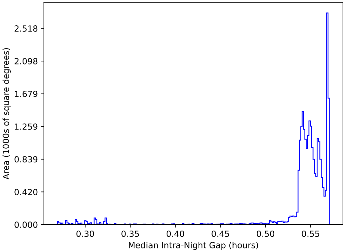
weather_cloudso10v3.4_10yrs All sky: Median Intra-Night Gap
