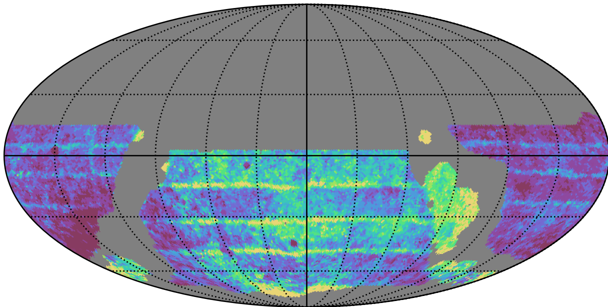
weather_cloudso10v3.4_10yrs WFD z band: Median Inter-Night Gap
