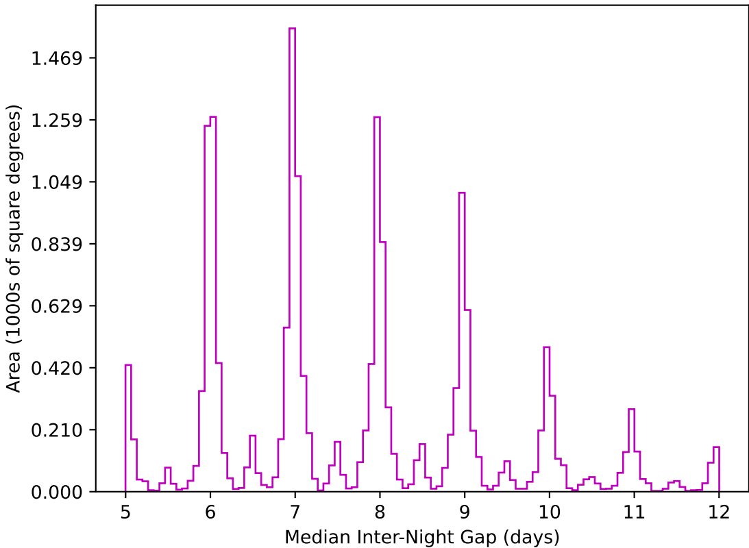
weather_cloudso10v3.4_10yrs WFD z band: Median Inter-Night Gap
