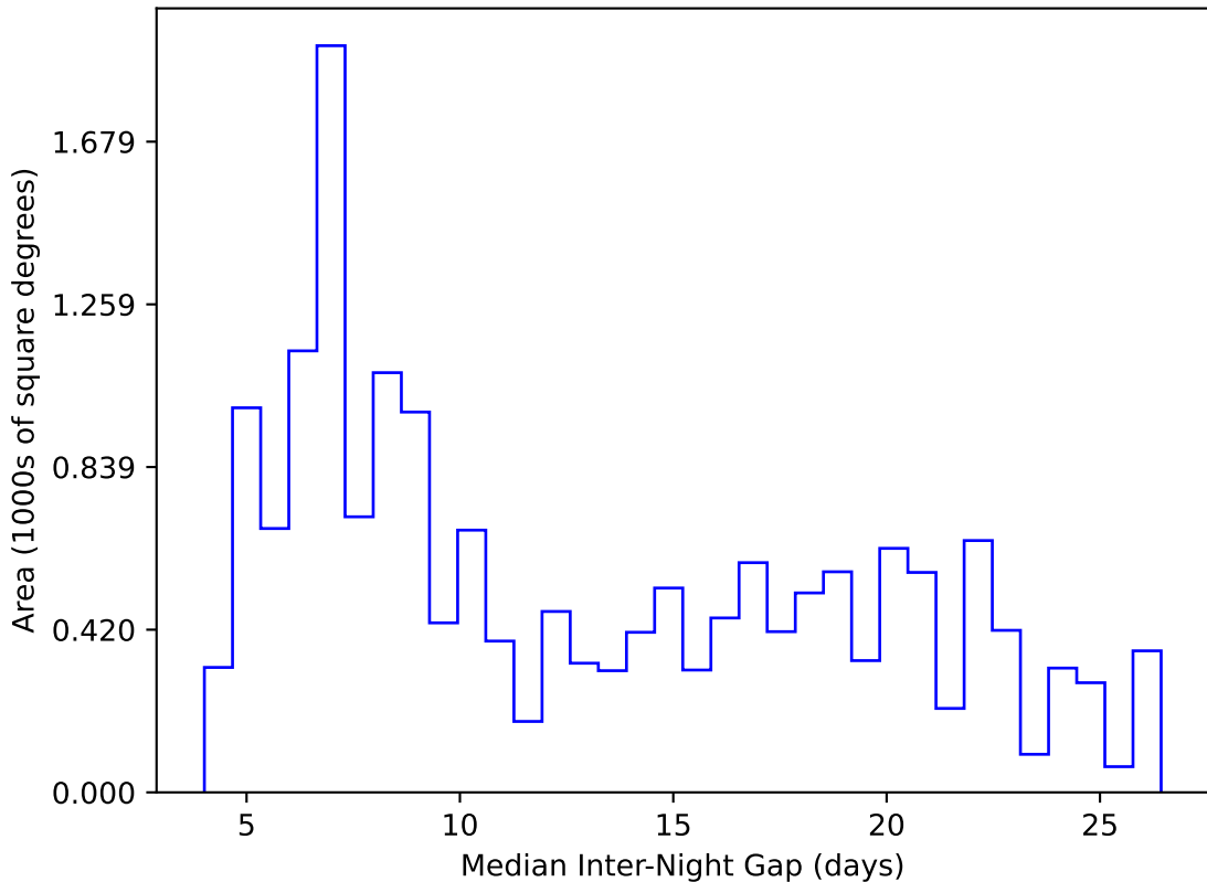
weather_cloudso10v3.4_10yrs WFD y band: Median Inter-Night Gap
