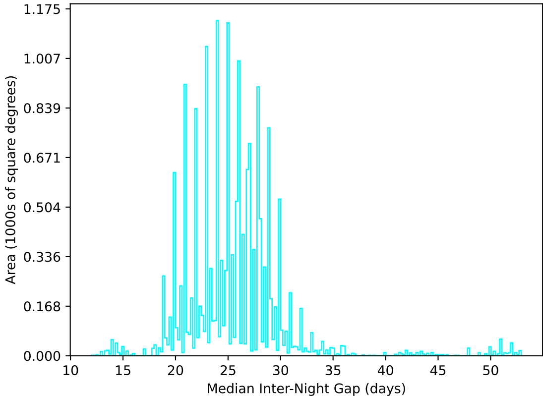
weather_cloudso10v3.4_10yrs WFD u band: Median Inter-Night Gap
