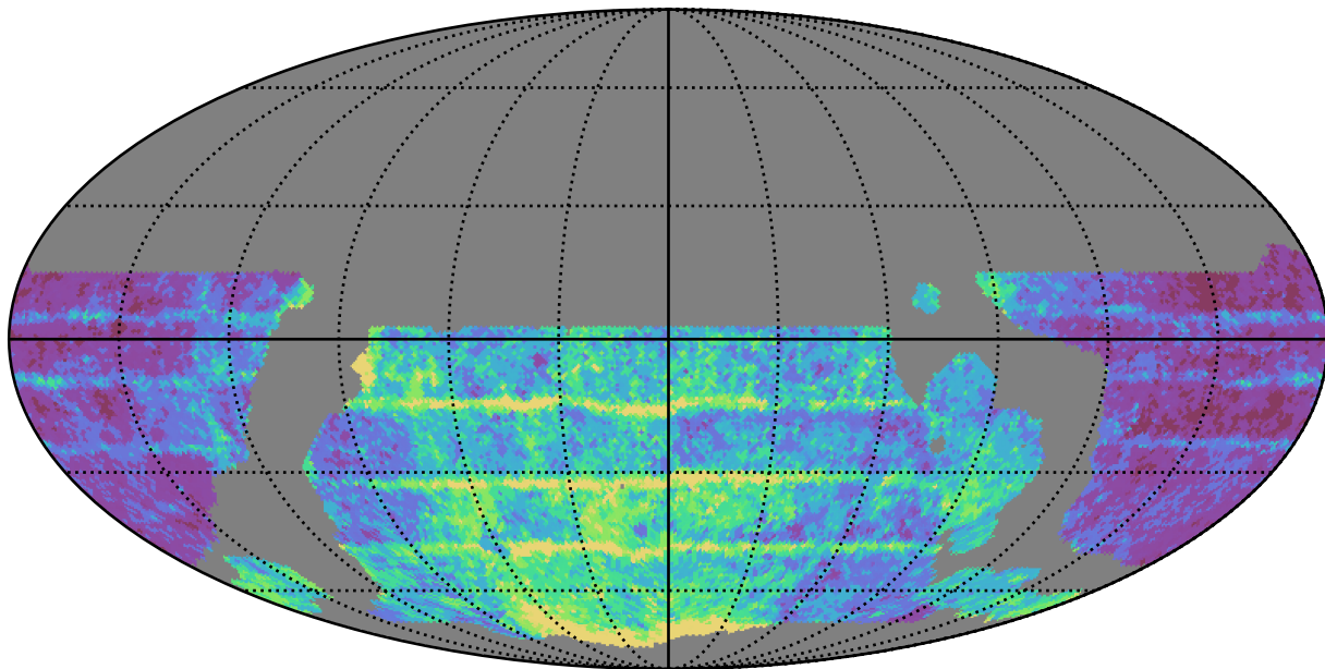
weather_cloudso10v3.4_10yrs WFD r band: Median Inter-Night Gap
