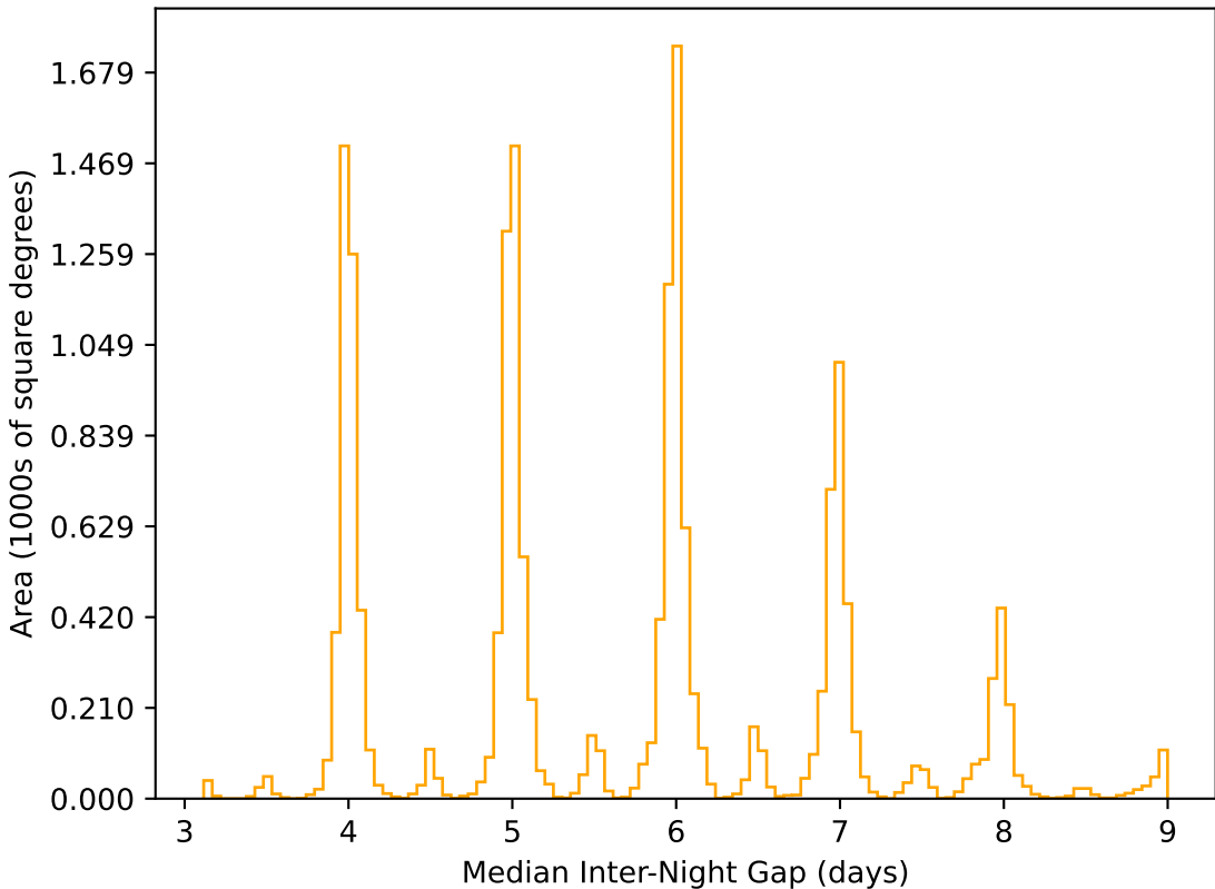
weather_cloudso10v3.4_10yrs WFD r band: Median Inter-Night Gap
