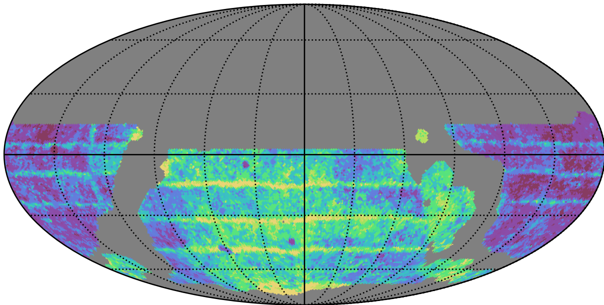
weather_cloudso10v3.4_10yrs WFD i band: Median Inter-Night Gap
