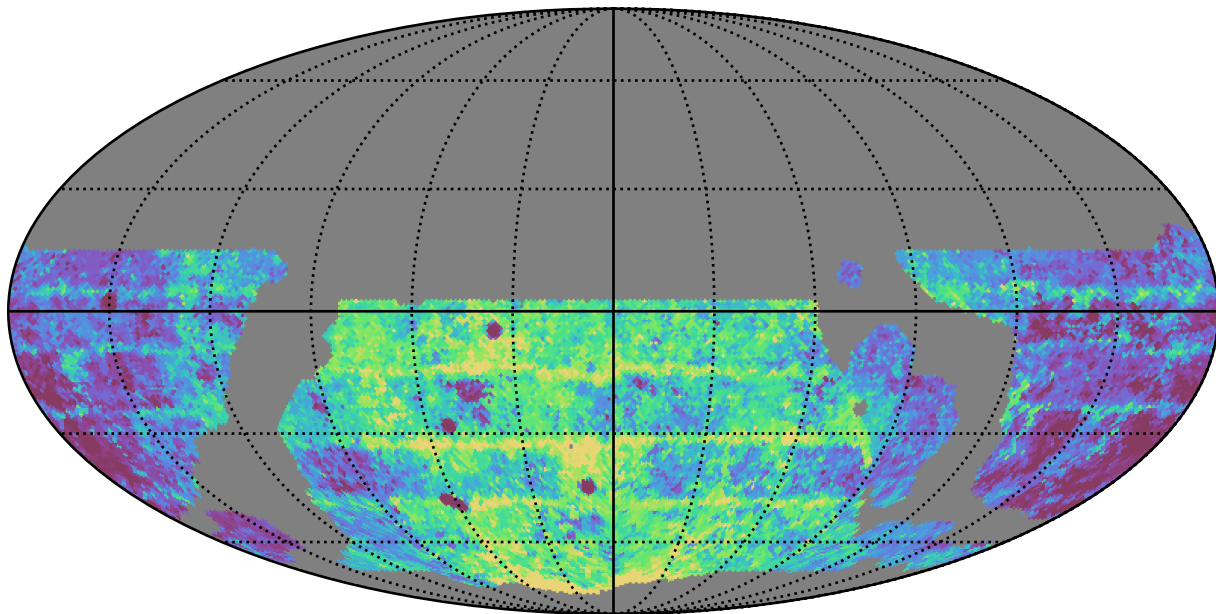
weather_cloudso10v3.4_10yrs WFD g band: Median Inter-Night Gap
