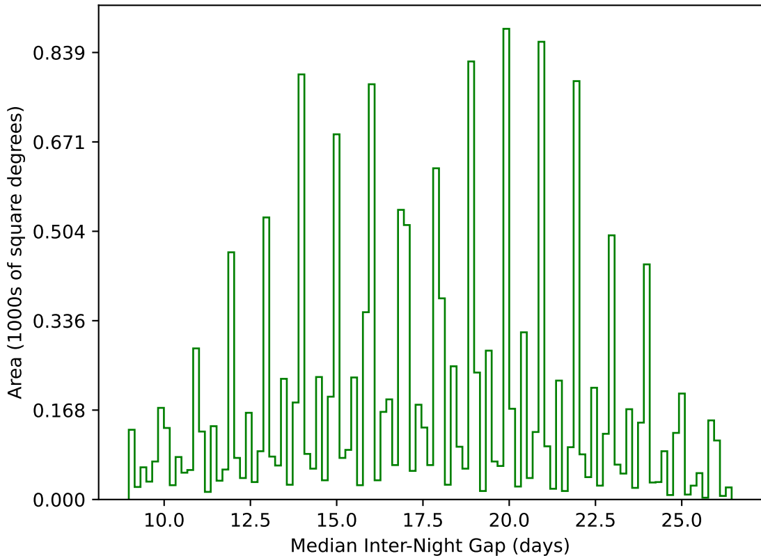
weather_cloudso10v3.4_10yrs WFD g band: Median Inter-Night Gap
