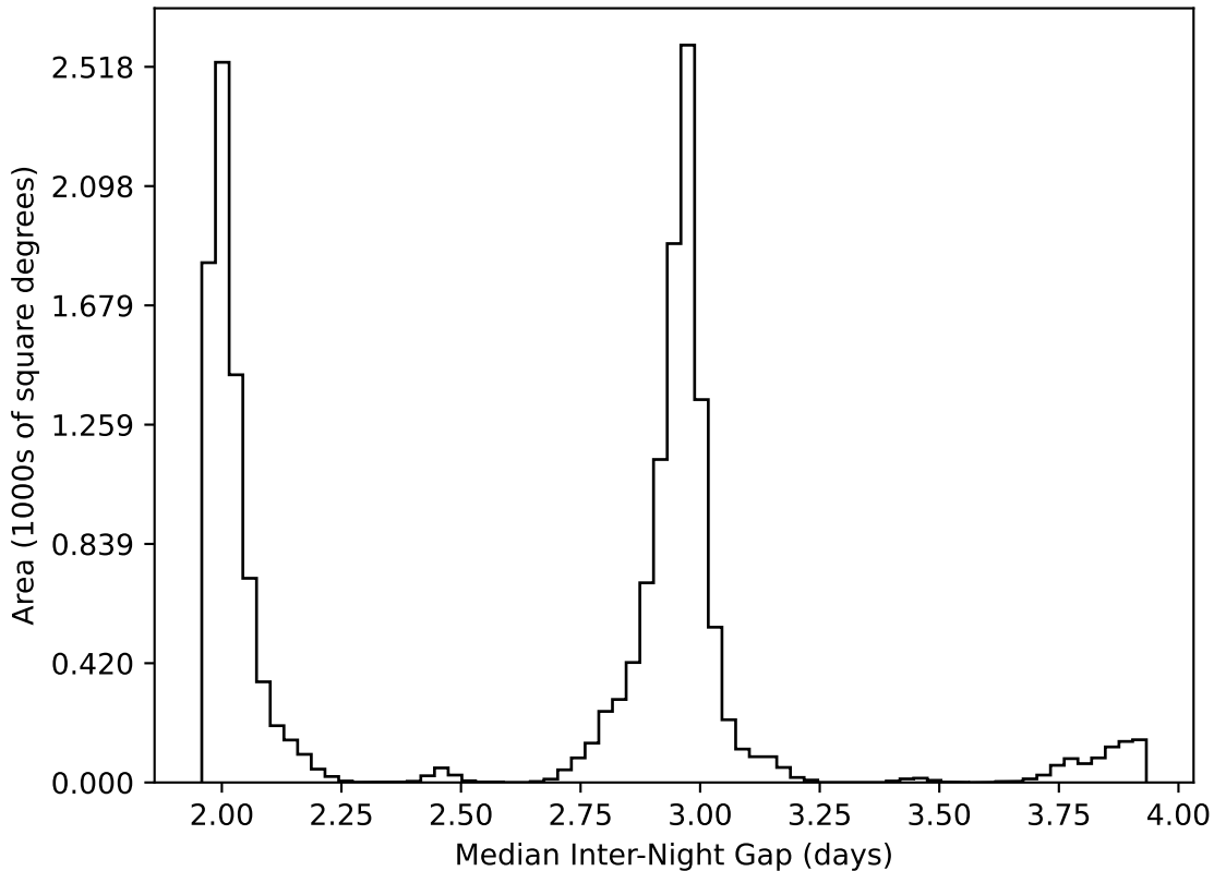
weather_cloudso10v3.4_10yrs WFD all bands: Median Inter-Night Gap
