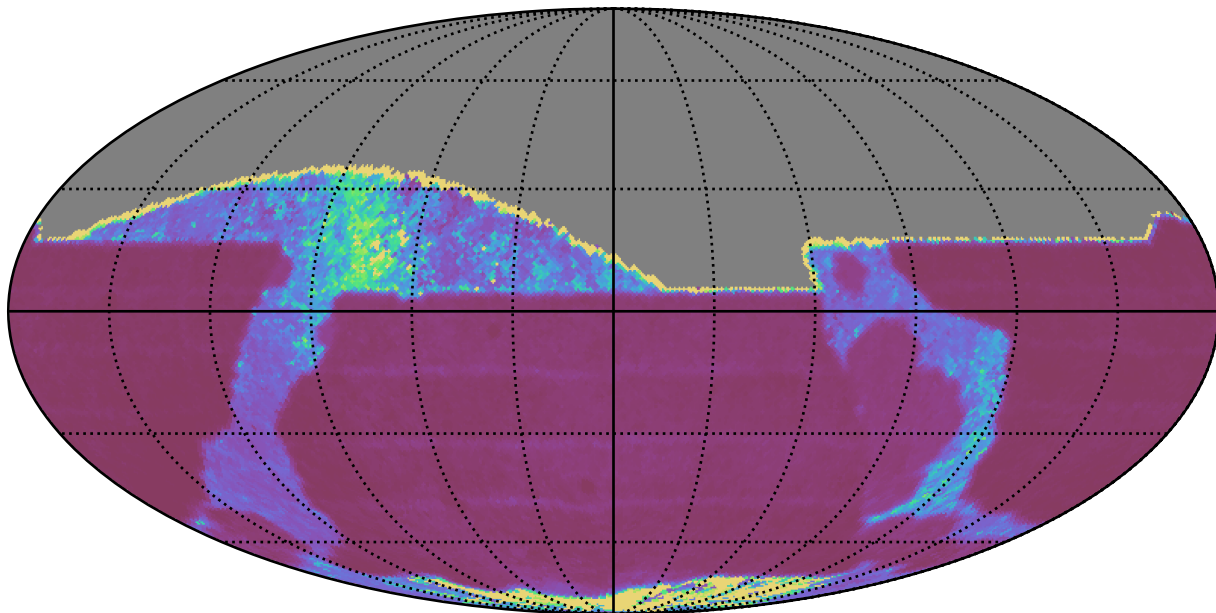
weather_cloudso10v3.4_10yrs All sky z band: Median Inter-Night Gap
