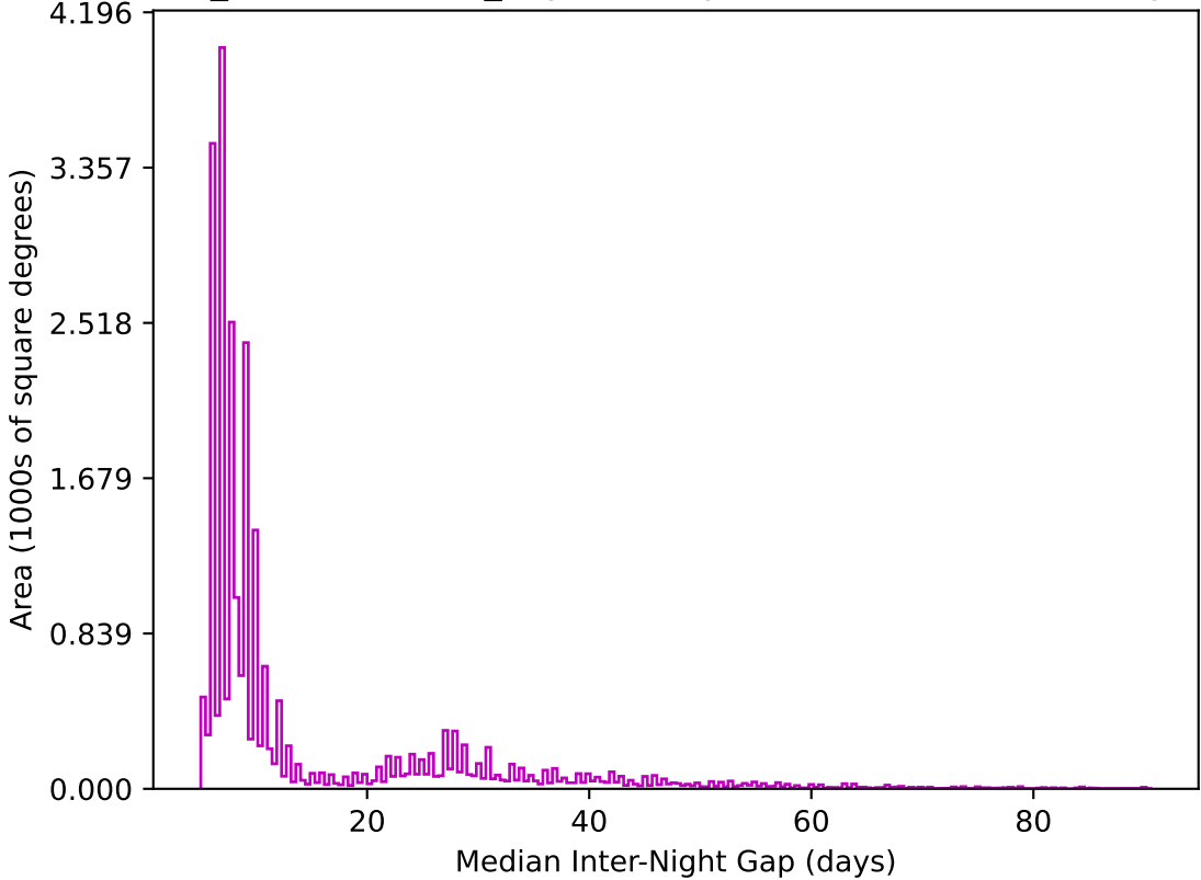
weather_cloudso10v3.4_10yrs All sky z band: Median Inter-Night Gap
