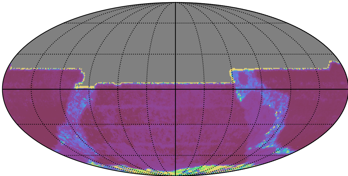
weather_cloudso10v3.4_10yrs All sky y band: Median Inter-Night Gap
