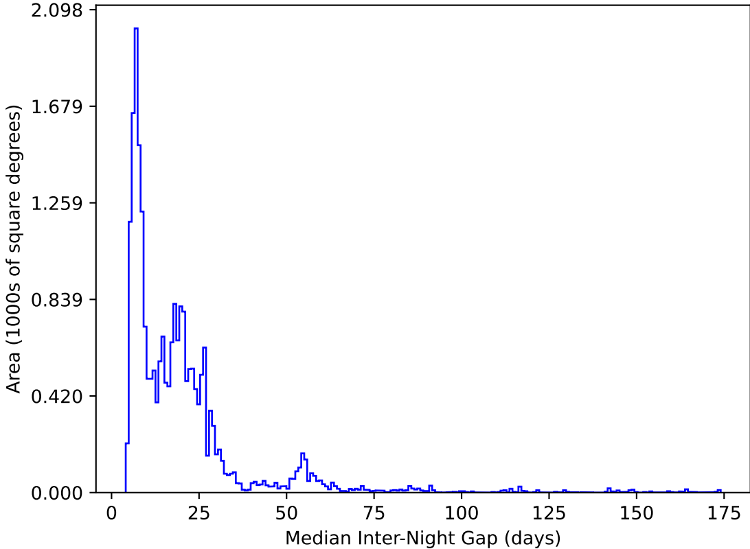
weather_cloudso10v3.4_10yrs All sky y band: Median Inter-Night Gap
