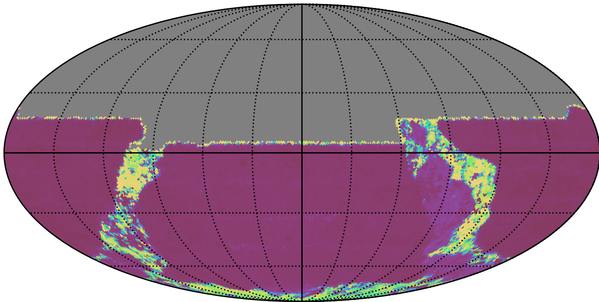
weather_cloudso10v3.4_10yrs All sky u band: Median Inter-Night Gap
