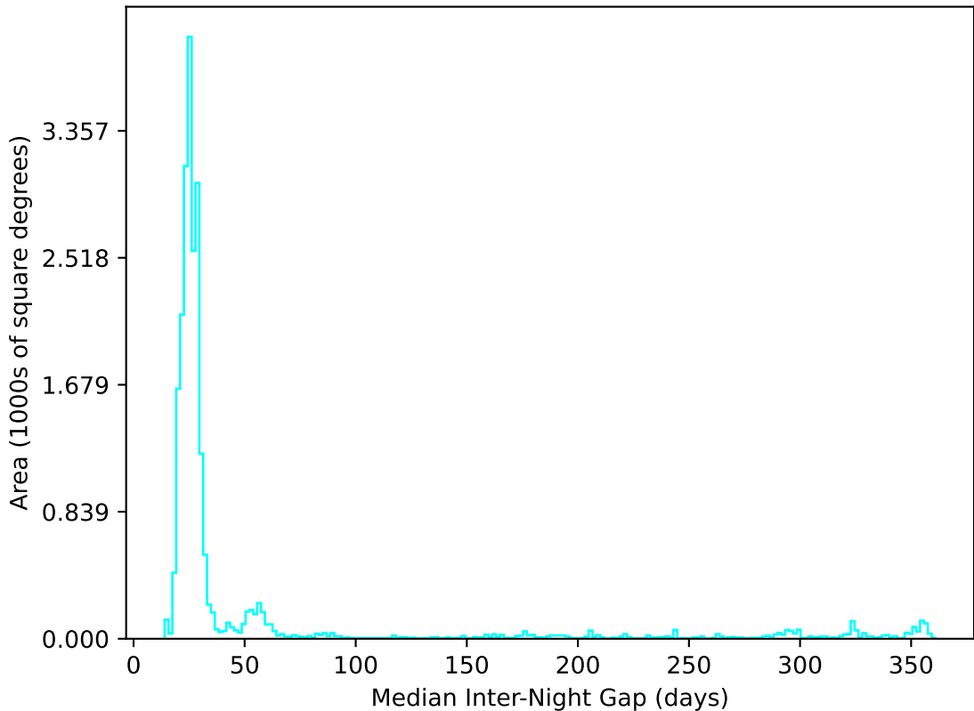
weather_cloudso10v3.4_10yrs All sky u band: Median Inter-Night Gap
