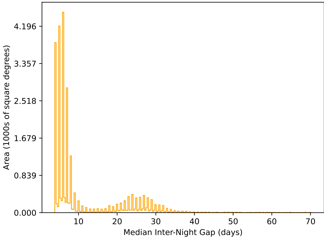
weather_cloudso10v3.4_10yrs All sky r band: Median Inter-Night Gap
