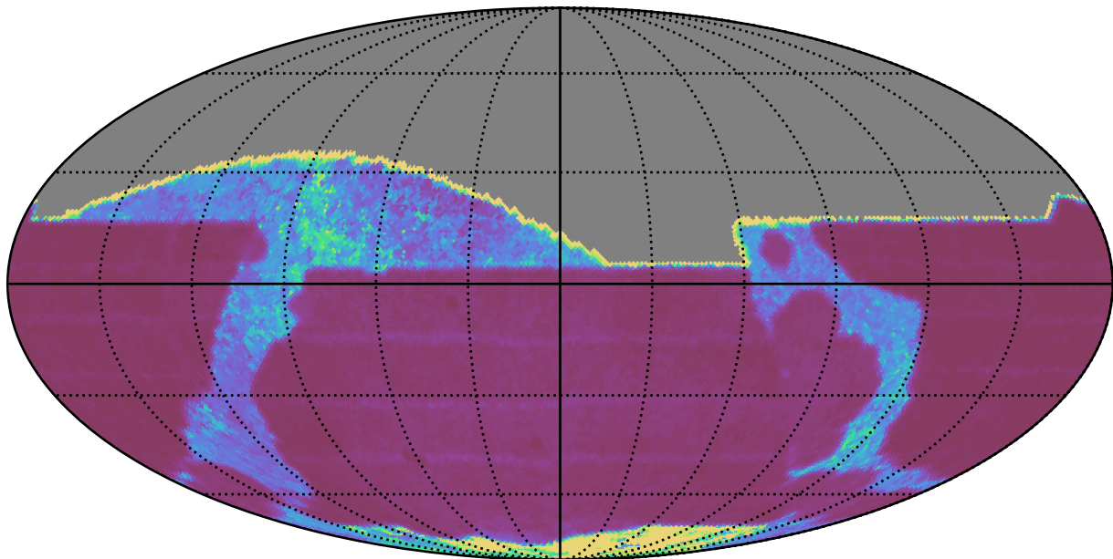
weather_cloudso10v3.4_10yrs All sky i band: Median Inter-Night Gap
