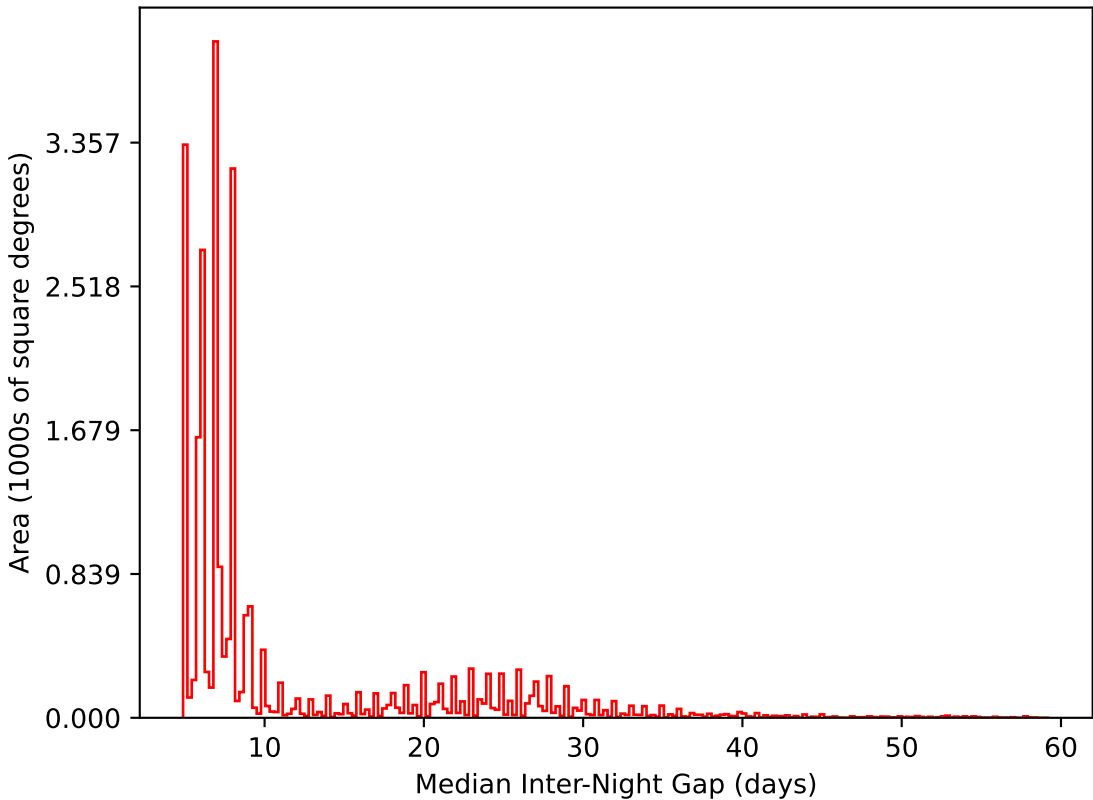
weather_cloudso10v3.4_10yrs All sky i band: Median Inter-Night Gap
