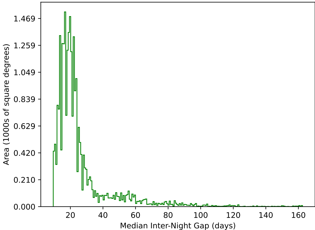
weather_cloudso10v3.4_10yrs All sky g band: Median Inter-Night Gap
