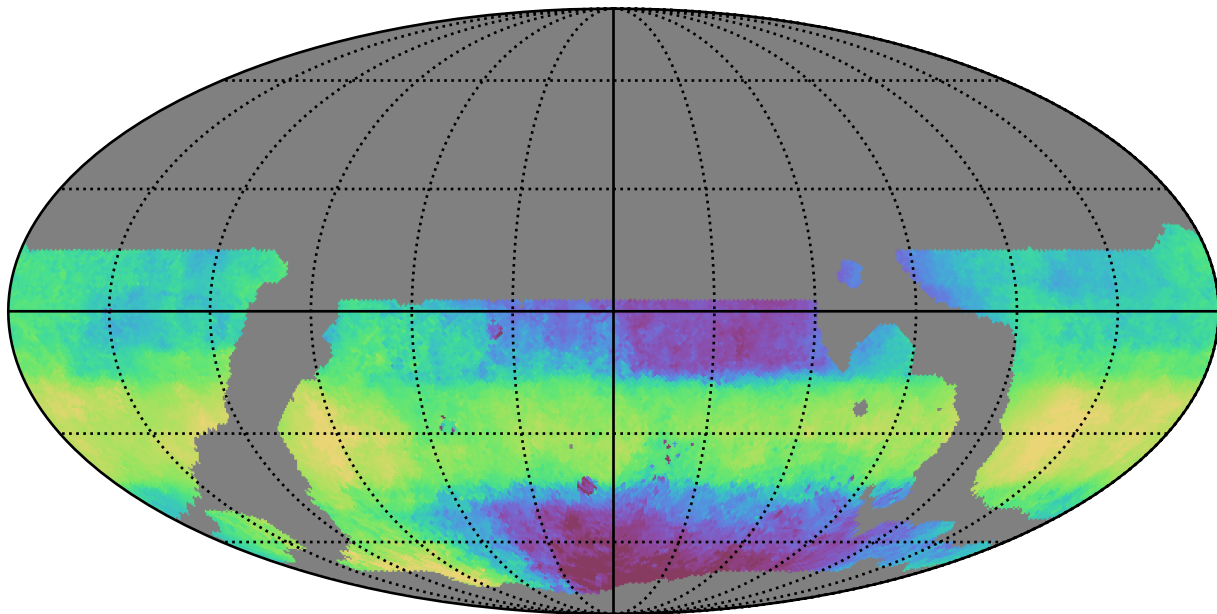
weather_cloudso10v3.4_10yrs WFD z band: Median HA
