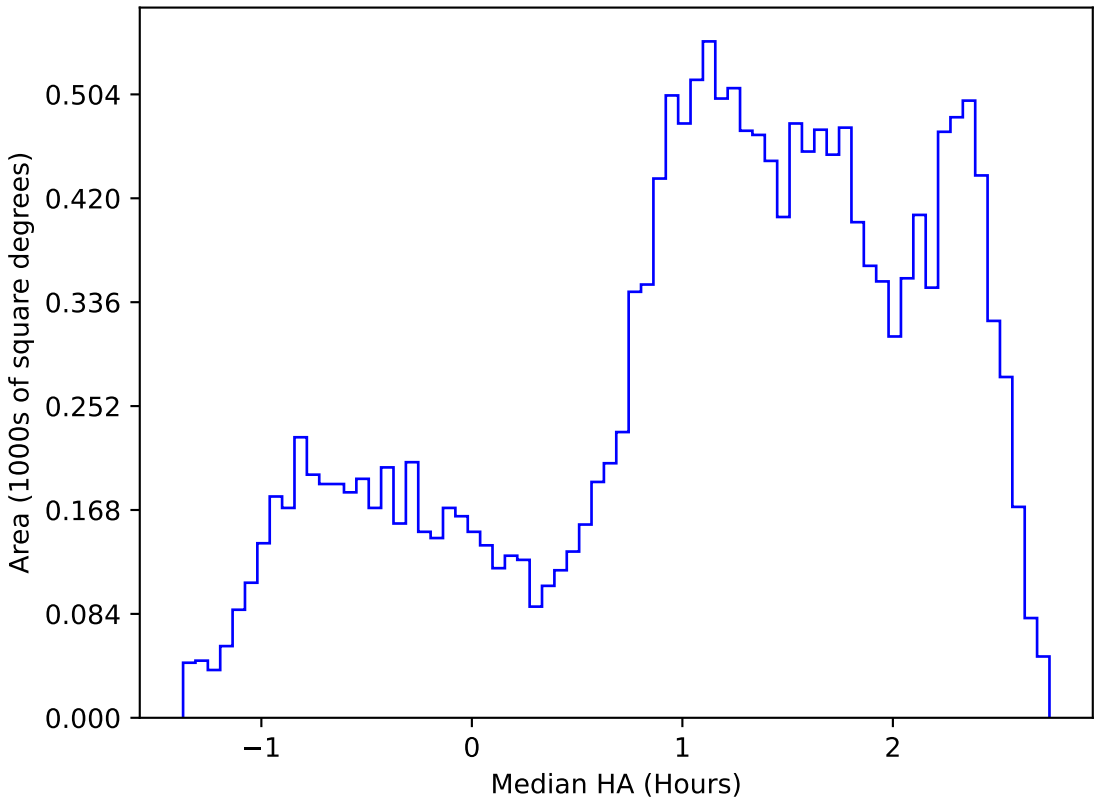
weather_cloudso10v3.4_10yrs WFD y band: Median HA
