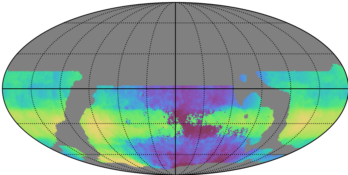
weather_cloudso10v3.4_10yrs WFD r band: Median HA
