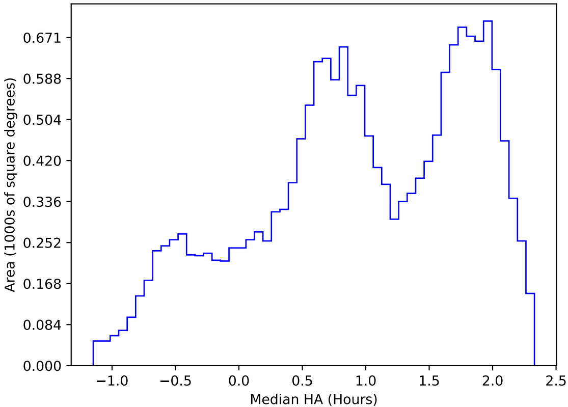
weather_cloudso10v3.4_10yrs WFD i band: Median HA
