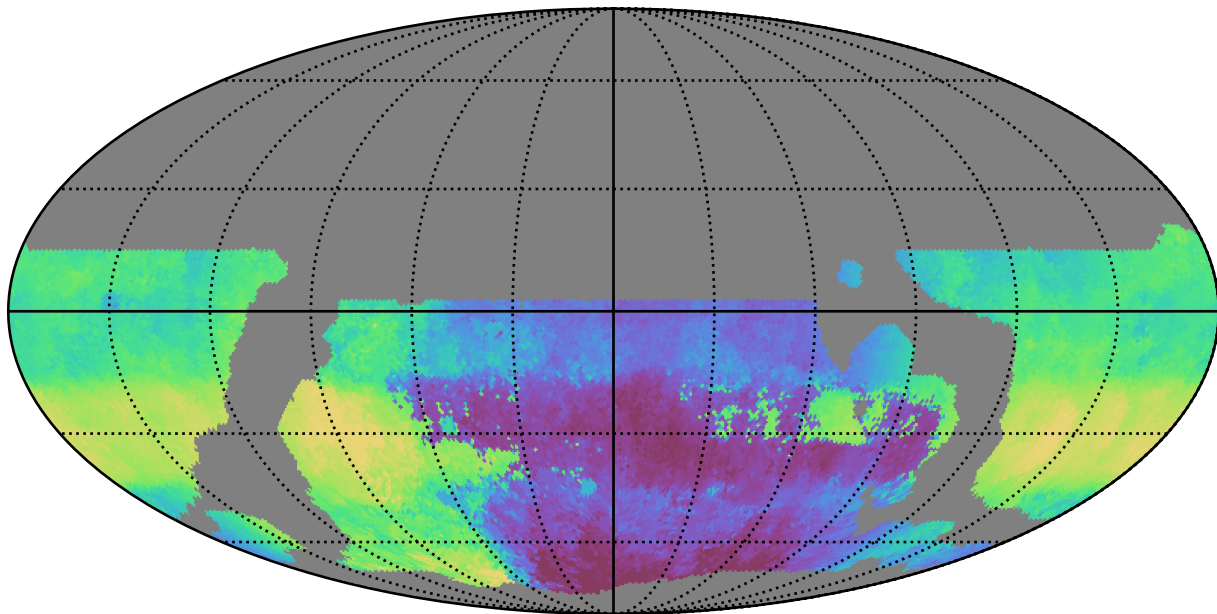
weather_cloudso10v3.4_10yrs WFD g band: Median HA
