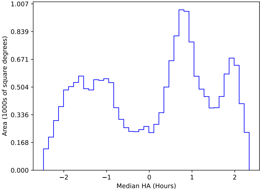
weather_cloudso10v3.4_10yrs WFD g band: Median HA
