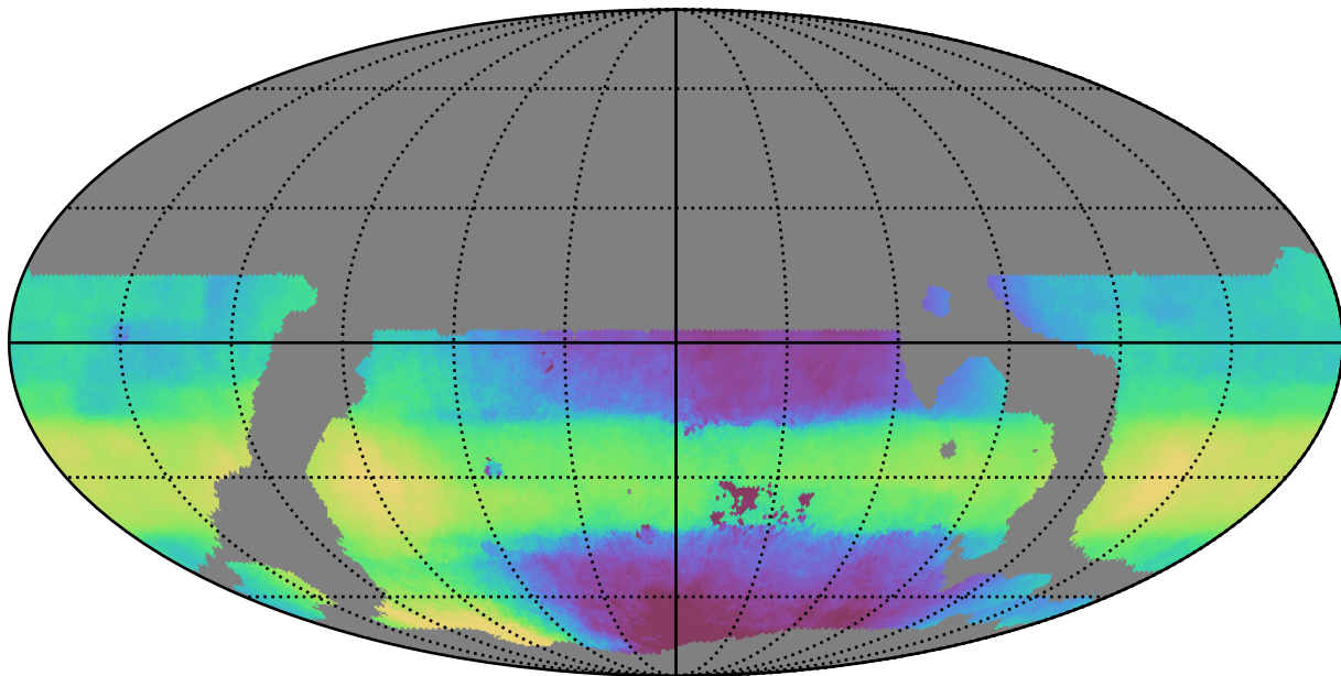
weather_cloudso10v3.4_10yrs WFD all bands: Median HA
