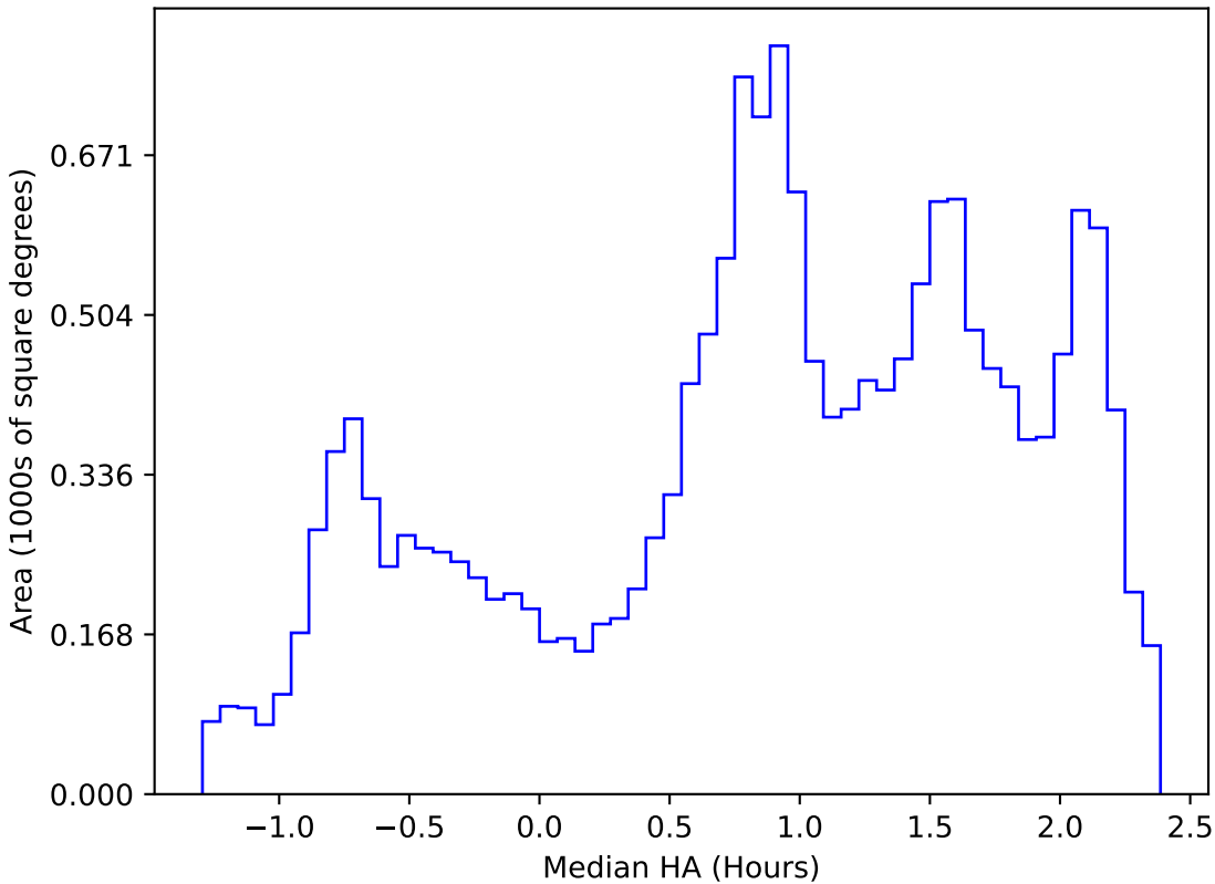
weather_cloudso10v3.4_10yrs WFD all bands: Median HA
