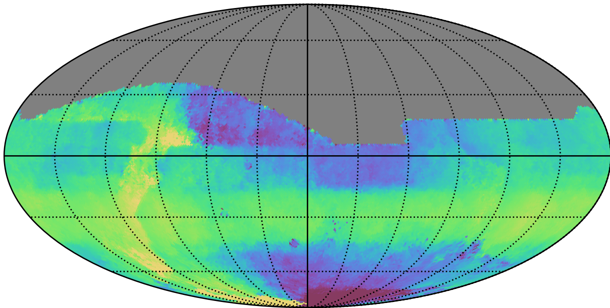
weather_cloudso10v3.4_10yrs All sky z band: Median HA
