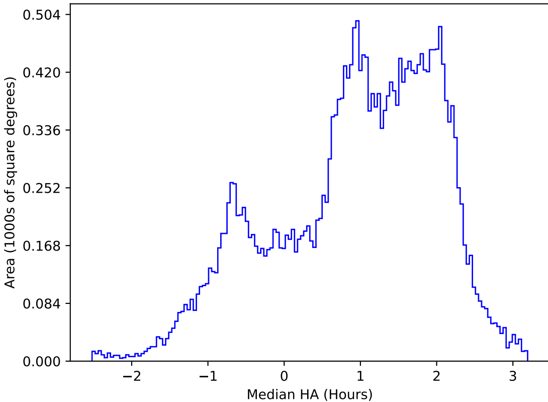
weather_cloudso10v3.4_10yrs All sky z band: Median HA
