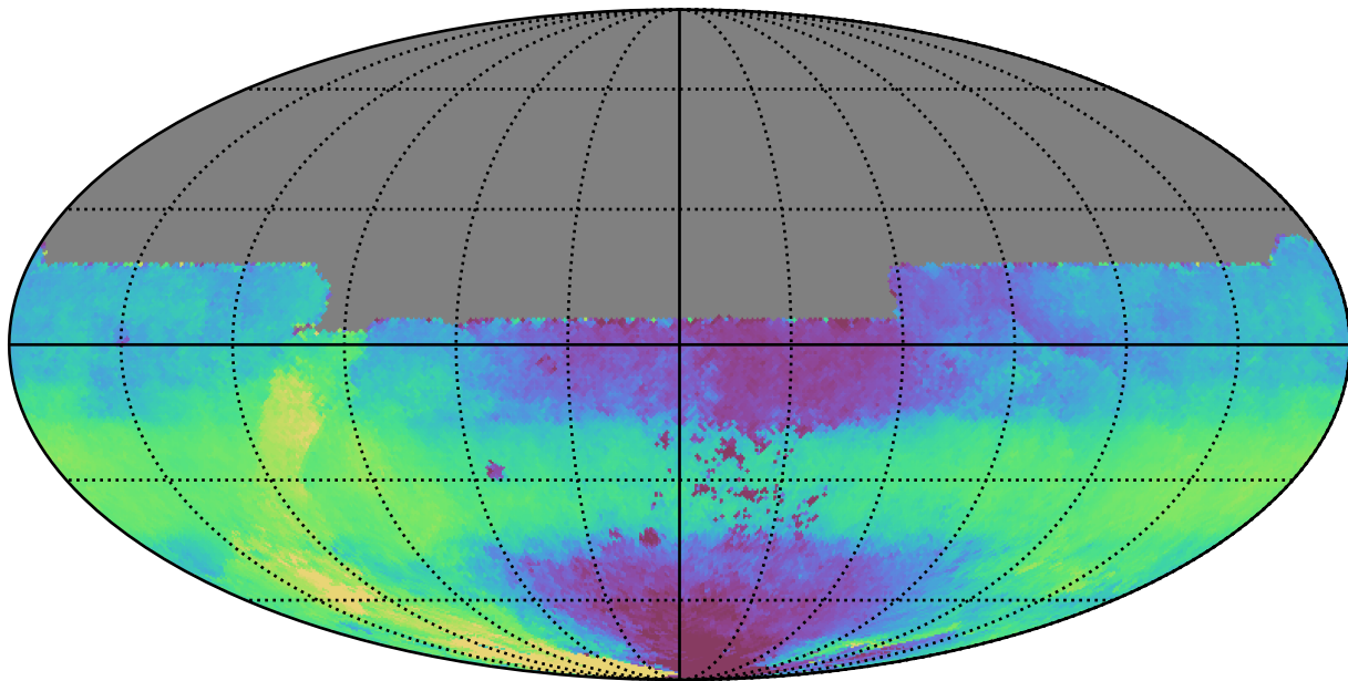
weather_cloudso10v3.4_10yrs All sky y band: Median HA
