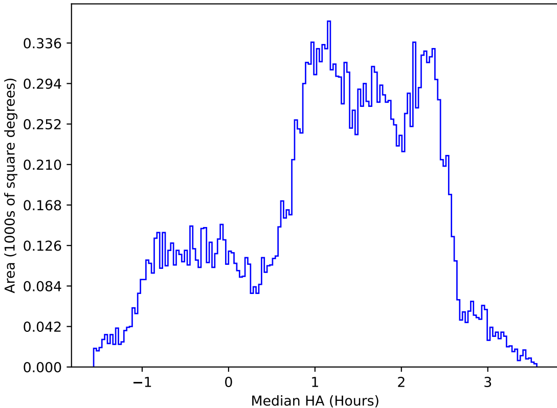
weather_cloudso10v3.4_10yrs All sky y band: Median HA
