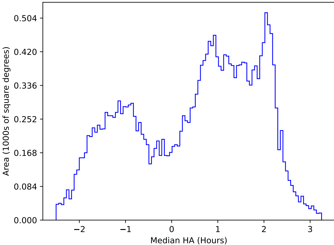
weather_cloudso10v3.4_10yrs All sky u band: Median HA
