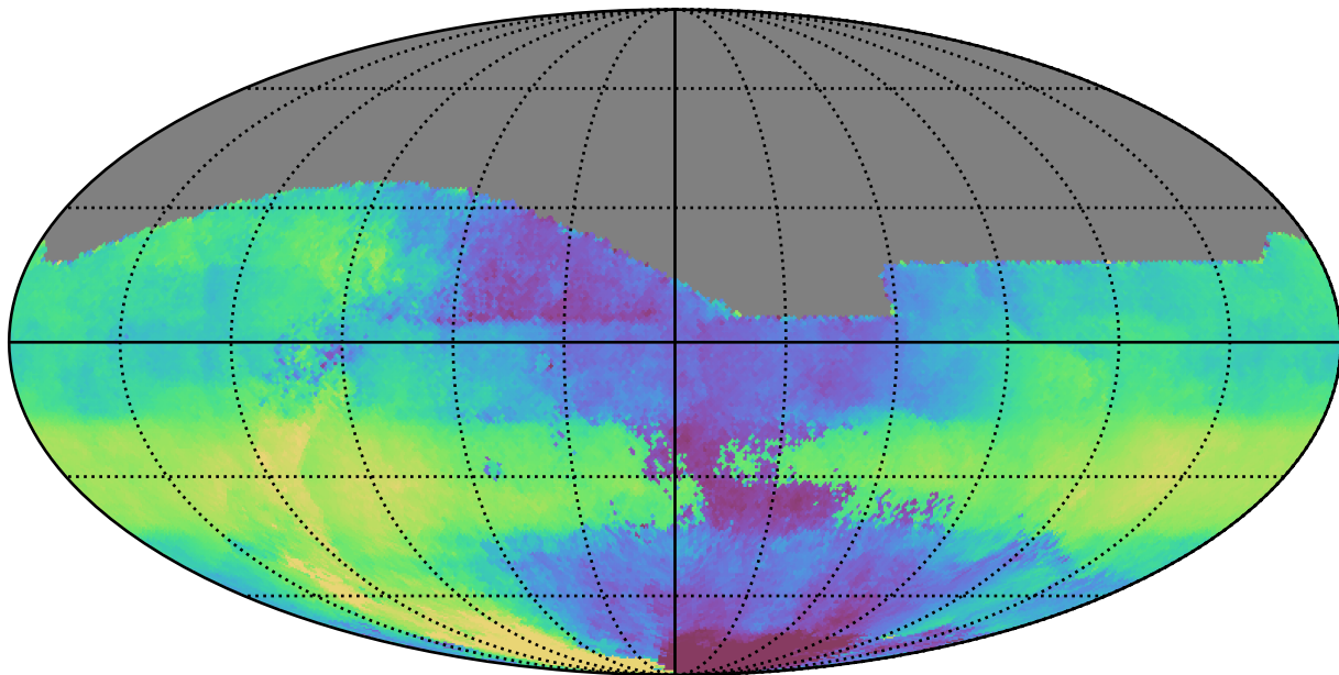
weather_cloudso10v3.4_10yrs All sky r band: Median HA
