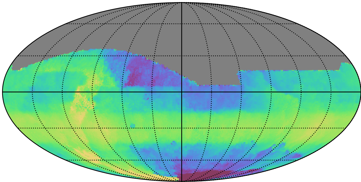
weather_cloudso10v3.4_10yrs All sky i band: Median HA
