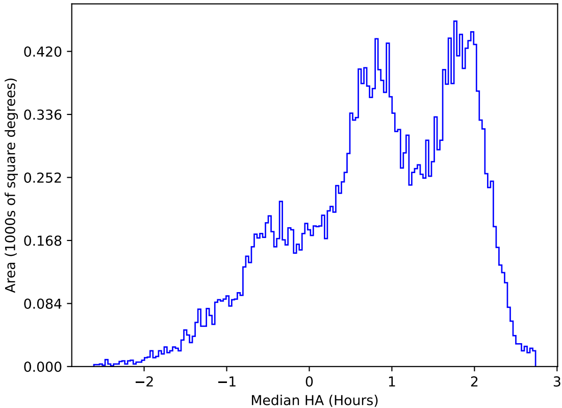
weather_cloudso10v3.4_10yrs All sky i band: Median HA
