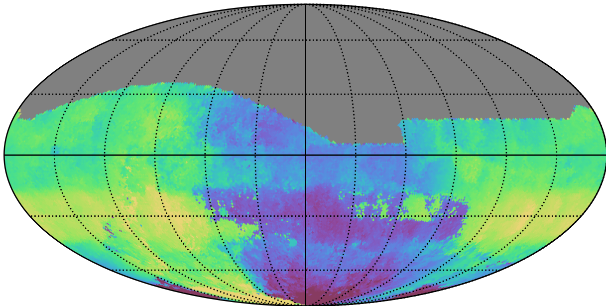
weather_cloudso10v3.4_10yrs All sky g band: Median HA
