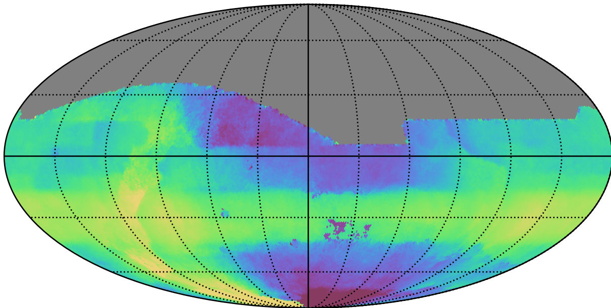
weather_cloudso10v3.4_10yrs All sky all bands: Median HA
